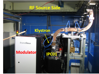
(a) RF source side: ScandiNova modulator, klystron, and IPC01 ion pump.
