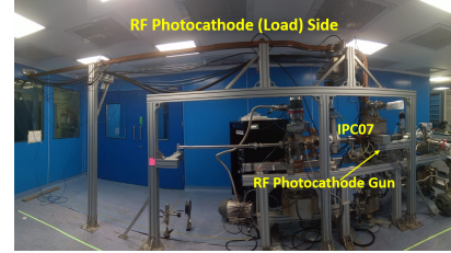
(b) Load side: RF photocathode gun and IPC07 ion pump.
