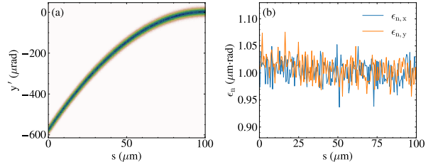
Figure 2: The distribution of (a) the angular kick y'(s) and (b) the normalized slice emittances at the exit of the HPC. Larger s corresponds to the bunch head.
