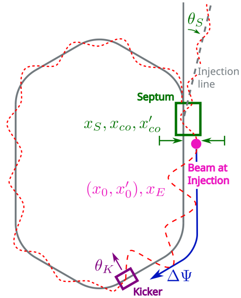
Figure 1: Schematic view of relevant parameters at injection.
