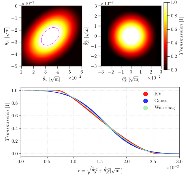
Figure 3: Top-left shows the transmission efficiency as function of (\tilde{\theta}_S, \tilde{\theta}_K) . The dashed ellipse shows the analytical solution for the "edge" transmission in comparison. Top-right shows the transmission as function of (\tilde{\theta}_S^*, \tilde{\theta}_K^*) once normalized. The bottom shows how well is the transmission related to radius r , hence defining a general function characterizing the injection efficiency.
