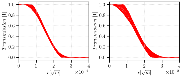
Figure 5: Including Chromaticity. Left) KV-Beam with a coherent momentum offset \delta = 1\% and a momentum spread of \Delta = \pm 2.5\% . Right) a KV-Beam with \delta = 0\% and \Delta = \pm 4\% .
