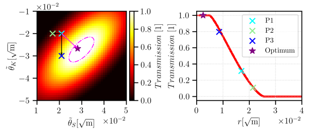
Figure 6: Example of the optimization procedure for the injection efficiency. The magenta arrow is the direction of optimization.
