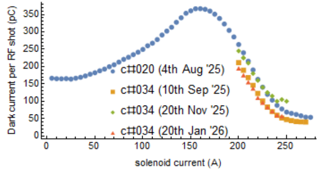
Figure 6: HRRG dark current measurement from the WCM vs. solenoid field strength, for different cathodes at different stages over the accelerator commissioning period. The gun power/gradient was set to the same value for all sets of data.
