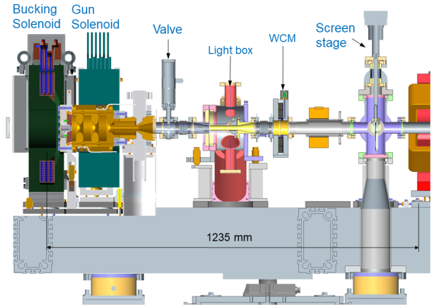
Figure 1: CLARA injector. WCM = wall current monitor.
