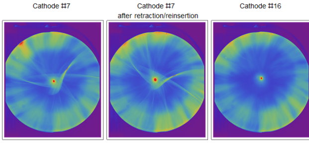
Figure 4: LRRG dark current on first beamline screen, with different cathode configurations.
