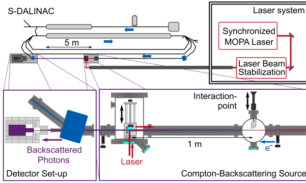
Figure 2: Layout of the COBRA setup installed in the third recirculation's straight section. Adapted from Ref. [11].
