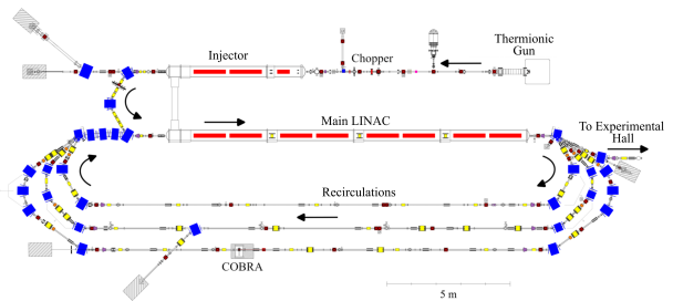
Figure 1: Floor plan of the S-DALINAC. The electron beam produced by a thermionic gun is first accelerated by the injector section and can be accelerated in the main LINAC up to four times due to the three recirculations. The COBRA setup is located in the third recirculation.
