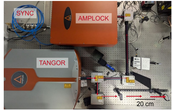
Figure 3: Labeled MOPA laser system for the external laser of the COBRA source, bought from Amplitude [12]. The path of the laser beam (red arrows) displays the small percentage of the beam used for the AMPLOCK and the telescope expanding the beam size for transport.
