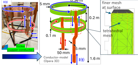
Figure 7: Kicker coil configuration, prototype, and OPERA-3D simulation model with surface-refined mesh.
