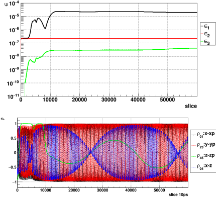
Figure 4: Evolution of eigen-emittances and correlation coefficients during the kicker.
