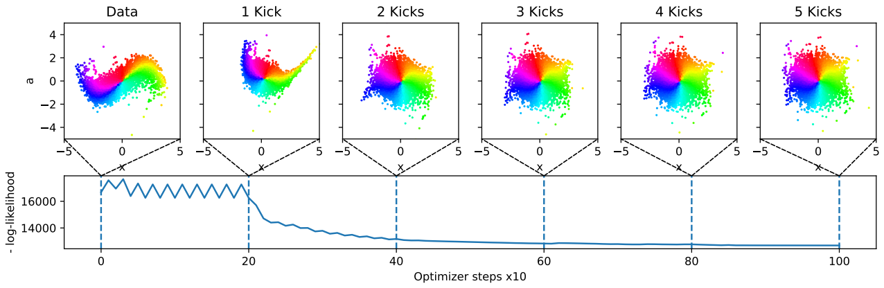
Figure 2: Layer-wise-optimization of the general Irwin model and its effect on a distorted distribution. To visualize the internal distortions, the points are colored according to the polar angle of the normal distribution from which the initial data was created.
