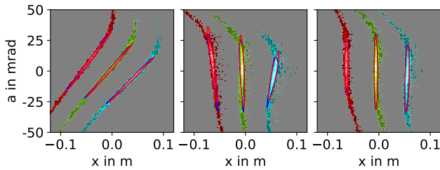
(a) Simulated large phase space. Initial, after QP optimization and after SP optimization.
