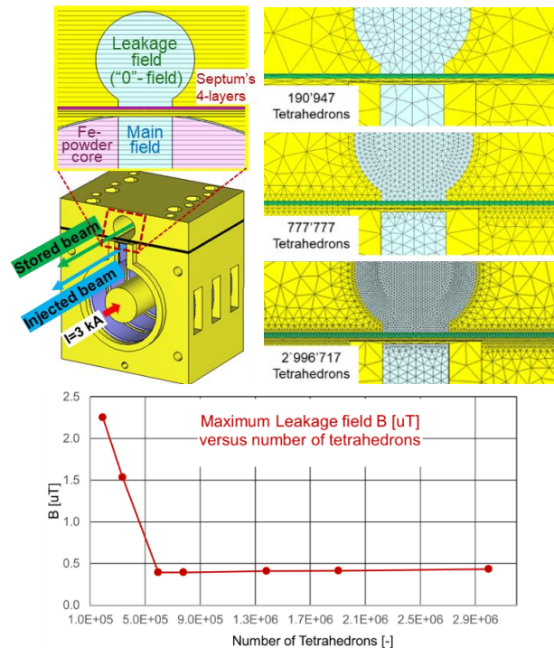
Figure 2: 3D CST® model and cross-section of a “sandwich” configuration with 4 layers used in parametric study (top left). Different mesh density based on different local meshing (top right). Influence of mesh size (number of tetrahedrons) on CST leakage field results (bottom plot) for thin septum excitation pulse of 3 kA amplitude.
