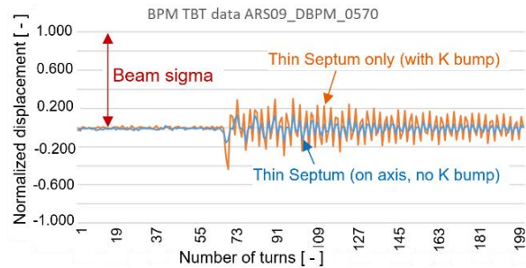
Figure 11: Normalized thin septum disturbance (beam sigma), orange – on the bumped orbit (bump kicker contribution subtracted) and blue - on axis (bump kicker off).
