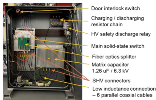
Figure 4: Thin septum pulser.
