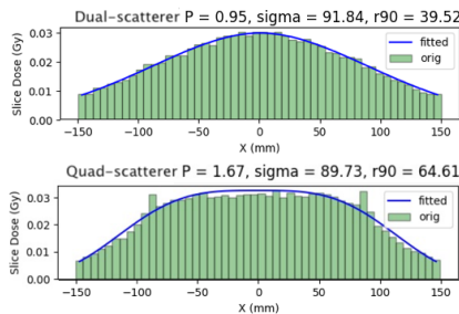
Figure 3: Comparison of the x dose distribution at 5 mm depth of a water phantom, of the dual-scattering system(top) and the quadrupole-scatterer system (bottom).
