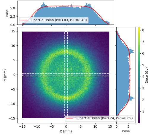
Figure 4: Current unoptimised dose profile of the CLEAR beam at 5 mm in the water phantom, with 10 nC of electrons.
