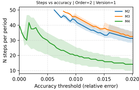
Figure 3: Median number of points (N) per period required to reach each accuracy threshold for O2/V1, comparing M2, M3, and M4. The shaded bands indicate the spread over the tested initial conditions.
