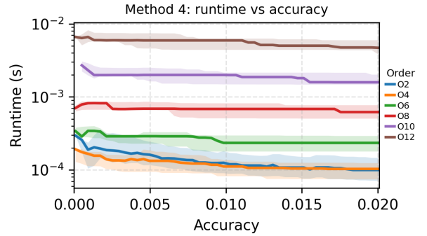
Figure 5: Median runtime required to reach each accuracy threshold for different integration orders in M4, combining both splitting versions. The shaded bands indicate the spread over the tested initial conditions.
