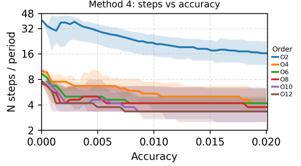
Figure 4: Median number of points (N) per period required to reach each accuracy threshold for different integration orders in M4, combining both splitting versions. The shaded bands indicate the spread over the tested initial conditions.
