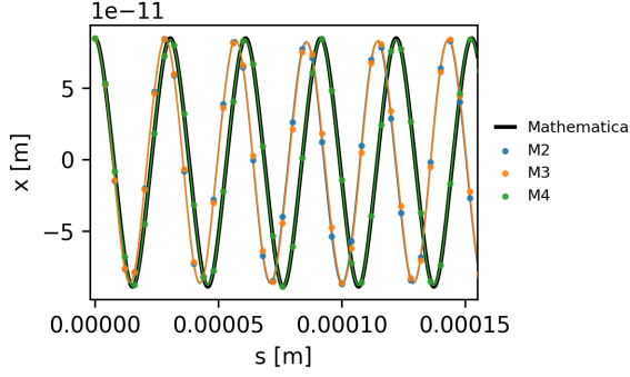
Figure 2: Comparison to the Mathematica solution for a given order/version (O2/V1), illustrating the better convergence of M4 in a low-step integration regime.
