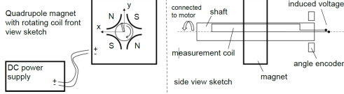
Figure 3: Rotating-coil measurement setup.
