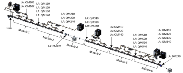
Figure 2: Placement of magnets along the ELI-GBS LINAC.
