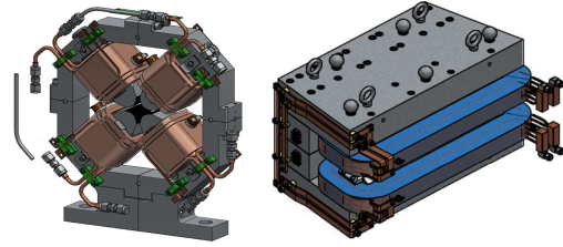
Figure 1: Views of the LINAC quadrupole and dipole.
