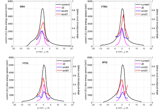
Figure 4: Current profiles, slice transverse normalized emittances and slice energy spread at the XFEL undulator entrance for four laser pulse shapes.
