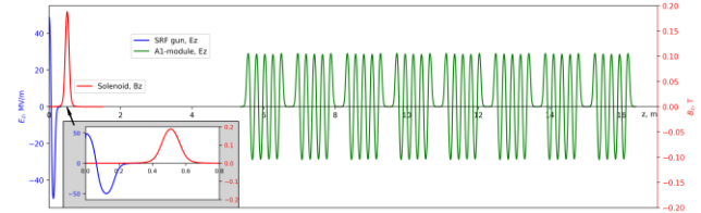
Figure 1: Electromagnetic field distribution along the SC photo injector.
