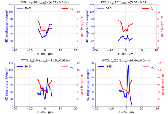
Figure 5: Local brightness and gain length distributions at the XFEL undulator entrance for four laser pulse shapes.
