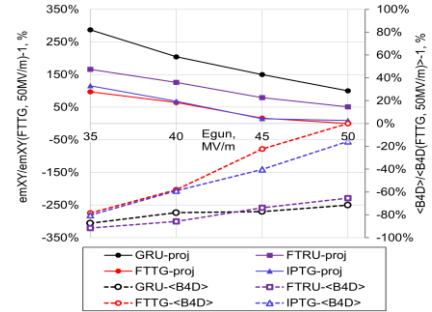
Figure 6: Electron beam performance at the photoinjector exit for various gun gradients.
