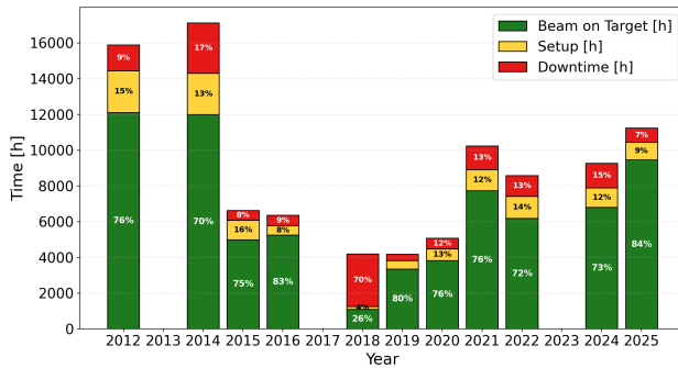
Figure 2: Evolution of GSI accelerators performance (2012 – 2025) based on OLOG – classified operational time.
