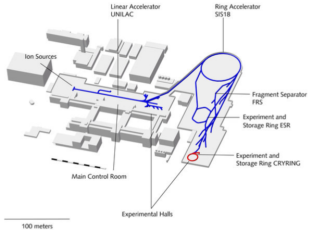
Figure 1: Overview of the GSI accelerator complex including the UNILAC injector linac, SIS18 synchrotron, ESR and CRYRING@ESR storage rings, transfer beamlines (HEST), and the connected experimental areas.
