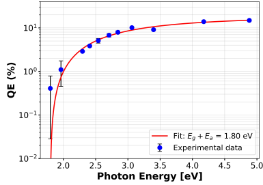
Figure 1: Spectral response of the NaKSb(Cs) photocathode (blue markers). The red curve represents the fit to the experimental data using Eq. (1).
