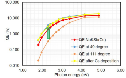
Figure 5: Spectral response of the NaKSb(Cs) photocathode at different stages of the thermal degradation study. The yellow curve corresponds to the spectral response after Cs rejuvenation.
