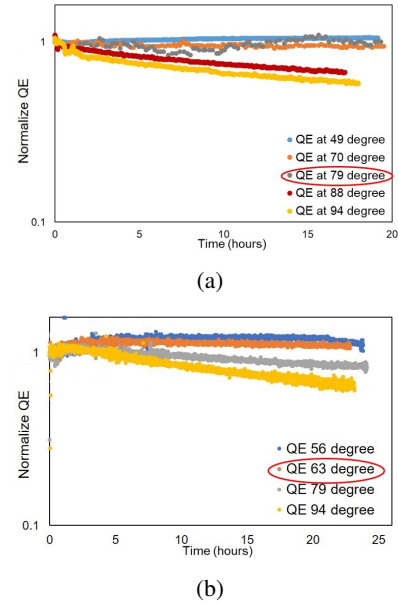
Figure 3: Decay curves of (a) NaKSb(Cs) and (b) KCsSb (thin) photocathodes measured at different substrate temperatures. The normalized QE is plotted on a logarithmic scale.
