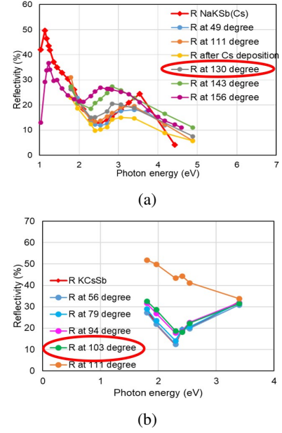
Figure 4: Spectral reflectivity of (a) NaKSb(Cs) and (b) KCSb (thin) photocathodes measured after thermal treatment at different substrate temperatures. For the KCSb photocathode, the spectral reflectivity was measured in the wavelength range from 365 nm to 690 nm due to experimental constraints.
