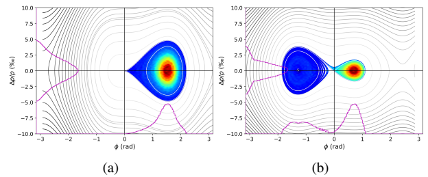
Figure 2: The evolution of particle distribution in the longitudinal phase space in hollow bunch method. (a) there is only one bucket with the second bucket has not been formed; (b) as the original bucket shrinks, the newly formed bucket become larger and is filled with low density particles.
