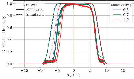
Figure 4: Normalised intensity vs. \delta for 3 chromaticity values, comparing simulation (dashed) and experiment (solid).
