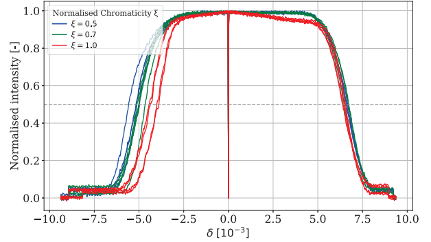
Figure 1: Normalised intensity vs. \delta measured in June 2025 for three values of normalised chromaticity \xi . A chromaticity dependence is observed only on the negative side.
