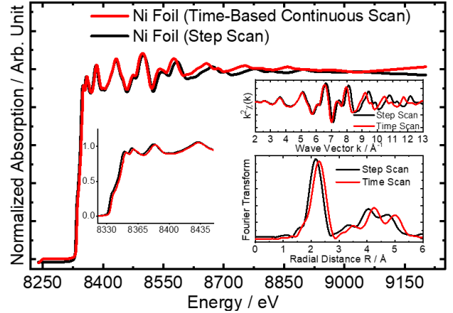
Figure 4: Ni K-edge (8333 eV) XAFS of Ni foil: step scan (black) vs. time-based continuous scan (red). Insets show the XANES region, k^2 \chi(k) , and Fourier transform of \chi(k) .
