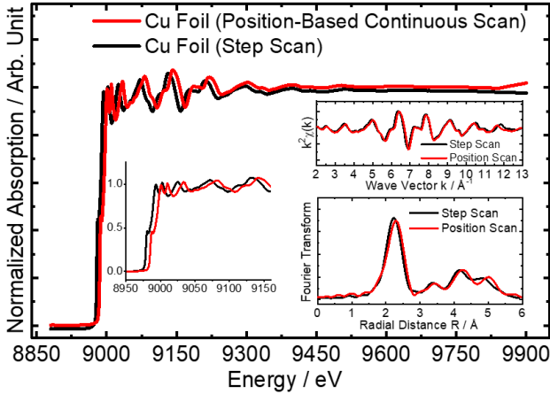
Figure 3: Cu K-edge (8979 eV) XAFS of Cu foil: step scan (black) vs. position-based continuous scan (red). Insets show the XANES region, k^2 \chi(k) , and Fourier transform of \chi(k) .
