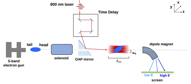
Figure 1: Schematic layout of the proposed experiment for validating relativistic ponderomotive dynamics. The laser–beam interaction takes place over an effective interaction length L_{\text{int}} near the laser waist w_0 .
