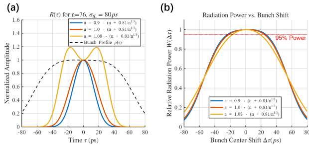
Figure 1: Numerical analysis of radiation characteristics: (a) normalized bunching factor R(\tau) under different modulation strengths a and bunch profile \rho(\tau) . (b) relative radiation power versus bunch shift \Delta\tau .
