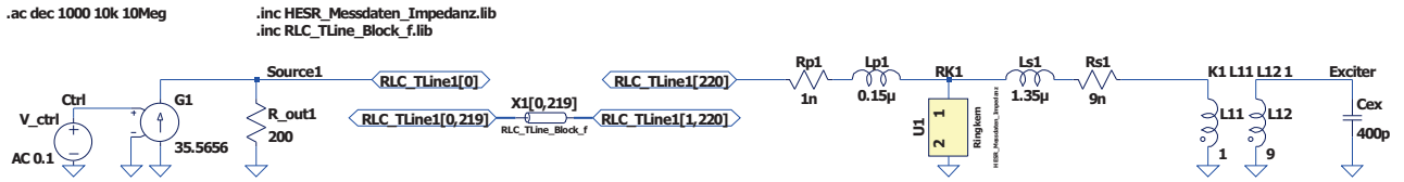
Figure 3: LTspice schematic of the reduced one-sided setup.
