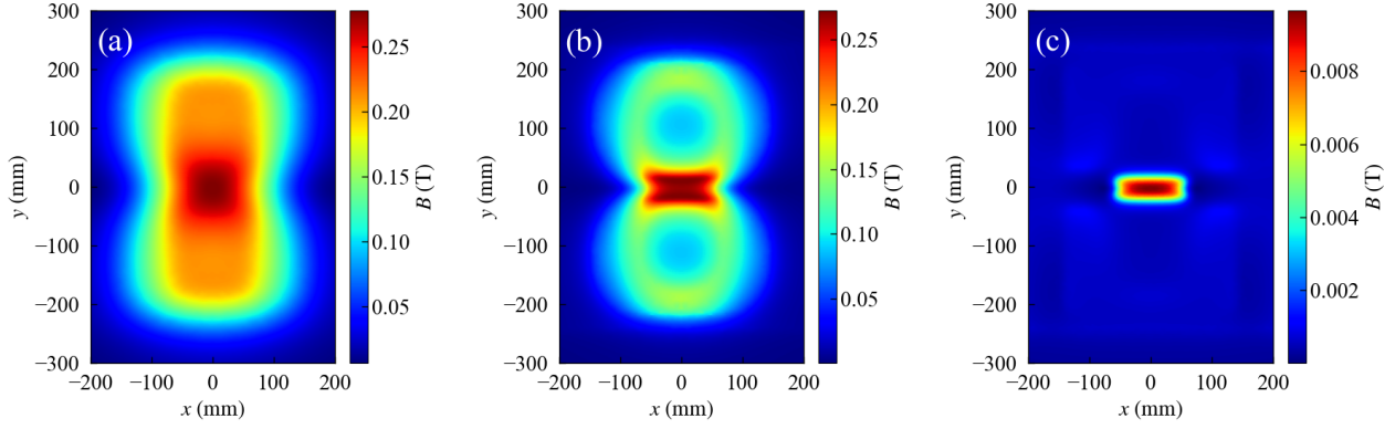
Figure 3: Leakage field distributions on the z = 260 mm plane near the surface of the PM-based dipole under three cases: (a) without magnetic shielding, (b) with the steel sheet shielding, and (c) with the proposed PM shielding.
