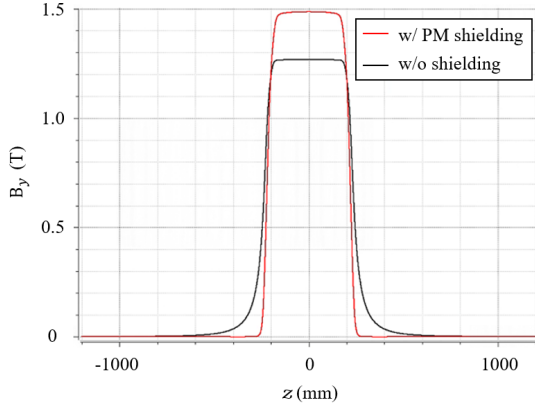
Figure 5: Longitudinal field distributions of the protective PM-based dipoles with the PM shielding (red line) and without magnetic shielding (black line).
