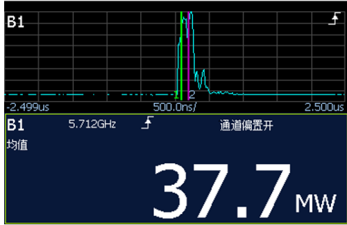
Figure 6: Output pulse waveform at the maximum power level.
