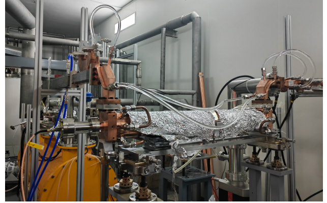
Figure 3: High-power tests in the C-band test platform.
