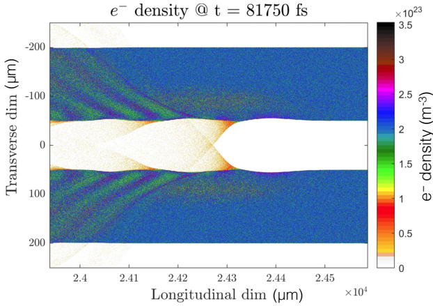
Figure 2: Simulation snapshot (after \approx 24\text{mm} of interaction) showing conduction electron density of crunch-in plasmon excited in a doped Silicon tube by an electron bunch with about 1.5nC charge, 30-micron overall dimensions.
