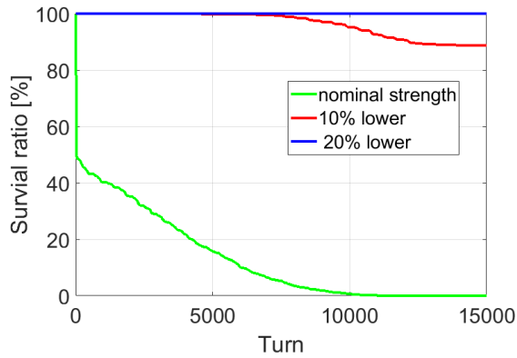
Figure 4: Survival ratios of the injected beam at different turns for the lattice cases with different octupole strengths.
