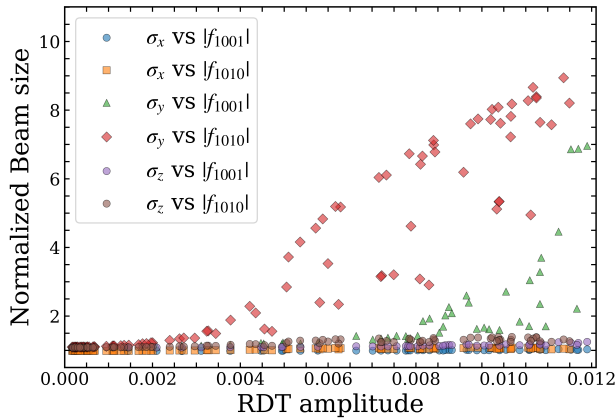
Figure 5: Normalized vertical and horizontal beam-sizes and bunch length vs. RDT amplitude at t\bar{t} .
