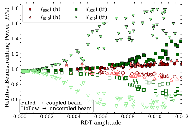
Figure 6: Normalized Beamstrahlung power of coupled and uncoupled beam vs. RDT amplitude at t\bar{t} and ZH, averaged over turns 800 to 1000.
