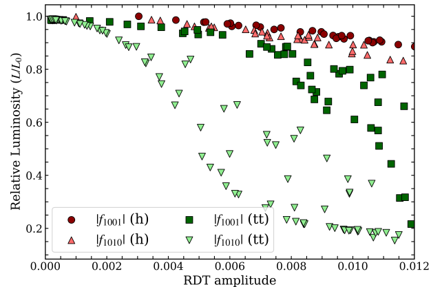
Figure 3: Luminosity dependence on |f_{1001}| and |f_{1010}| at ZH and t\bar{t} , with full beam beam. The luminosity was averaged over turns 800 to 1000 and normalized to the value at zero coupling.
