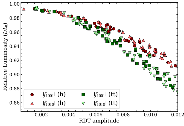
Figure 4: Luminosity dependence on |f_{1001}| and |f_{1010}| at the t\bar{t} and ZH working points, with the beam-beam strength enormously reduced by a factor of 10^9 . The luminosity was averaged over turns 800 to 1000 and normalized to the value at zero coupling.
