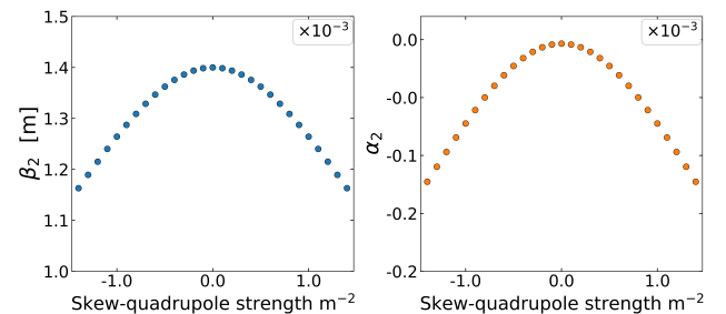
Figure 1: The IP normal mode functions \beta_2 and \alpha_2 versus the strength of two skew quadrupoles (of opposite sign) inserted in the full lattice after the crab sextupoles on either side of the IP, in the absence of any beam-beam element.
