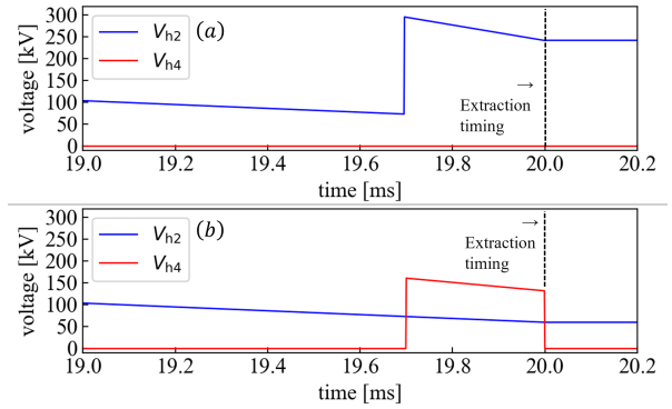
Figure 9: Voltage patterns that minimize the bunch width while keeping the \pm \Delta p/p peak below the limit ( \approx 1 %). (a) only the fundamental RF voltage; (b) with second harmonic RF superimposed.
