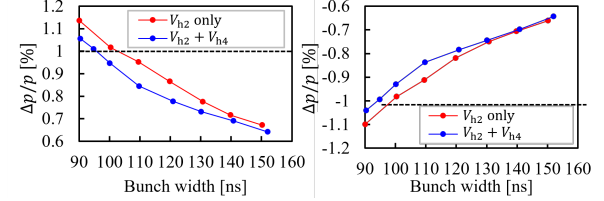
Figure 8: The peak of \pm \Delta p/p for final bunch widths of 150, 140, 130, ..., 90 (i.e., 10 ns increments) at RCS extraction.
