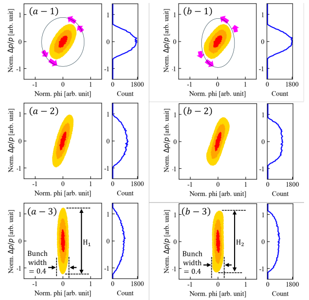
Figure 5: Comparison of the bunch shortening process using only the fundamental RF voltage (left column) and with second harmonic superposition (right column). Time progresses from top to bottom.
