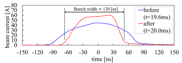
Figure 2: WCM measurements before the bunch shortening operation (blue) and of the shortened extraction beam (red).
