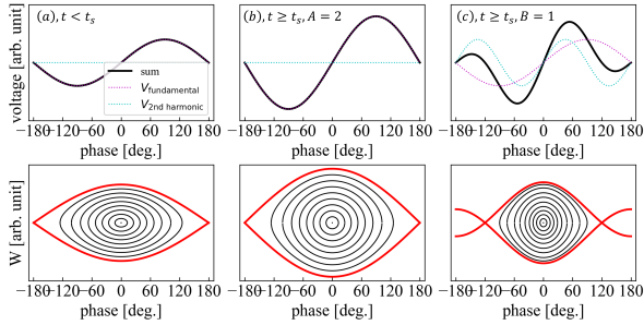
Figure 3: Comparison of voltage waveforms and separatrix shapes during the bunch shortening operation. (a) before the operation, (b) with the only fundamental RF voltage, (c) with the second harmonic RF voltage superimposed.
