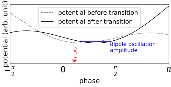
Figure 2: Longitudinal potential in the EAST bucket before and after transition crossing. The bottom of the potential well moves almost instantly at transition. Therefore, the EAST bunch becomes offset with respect to its potential well. Beam induced voltage from both bunches is accounted for in the potential.
