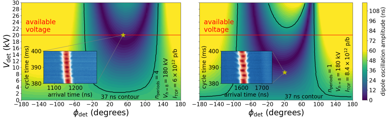
Figure 4: Estimated amplitude of residual dipole oscillations when detuning one of the main cavities to compensate the difference in beam induced voltage. The left contour shows the configuration where the bunch spacing and TOF intensity is unchanged from Table 1. The right contour shows the configuration where the bunch spacing is reduced and TOF intensity increased. The compensation scheme necessarily decreases the voltage on the principal harmonic to V_{h=8} = 180 kV. All parameters other than n_{\text{periods}} , I_{\text{TOF}} , and V_{h=8} are taken from Table 1. The black line indicates the dipole oscillation amplitude observed in Fig. 1 corresponding to the settings in Table 1. The insets show measured mountain range plots of the EAST bunch at transition close to the expected ideal settings of phase and voltage for the detuned cavity.
