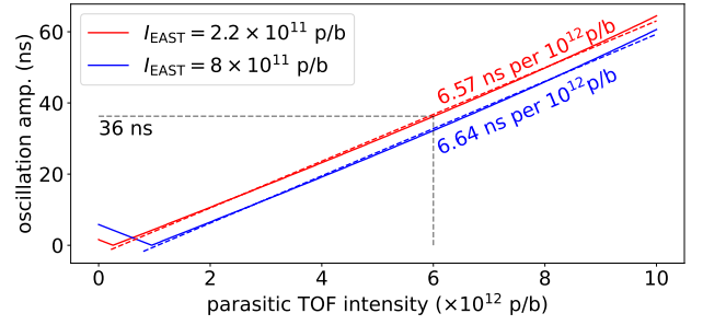
Figure 3: Expected dipole oscillation amplitude calculated using the parameters in Table 1, but varying TOF and EAST intensities. Linear fits and their gradients are overlaid.
