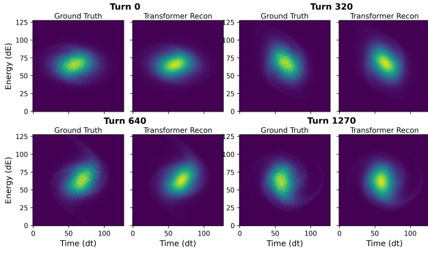
Figure 2: Snapshots of the longitudinal phase space evolution. For each specified turn, the ground truth (left) is compared with the Transformer reconstruction (right).
