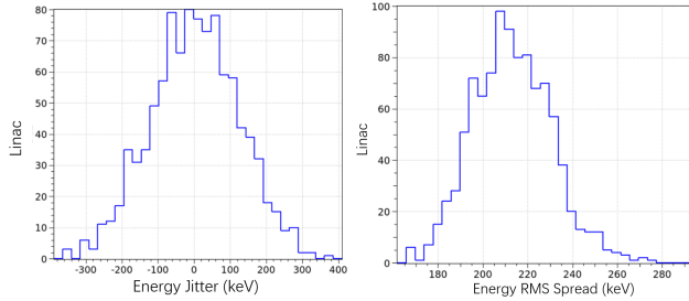
Figure 2: The error analysis considering all rf cavities errors for 1000 random machines. The left hand side plot shows the distribution of \Delta E and the right hand side plot shows the information about the energy spread.
