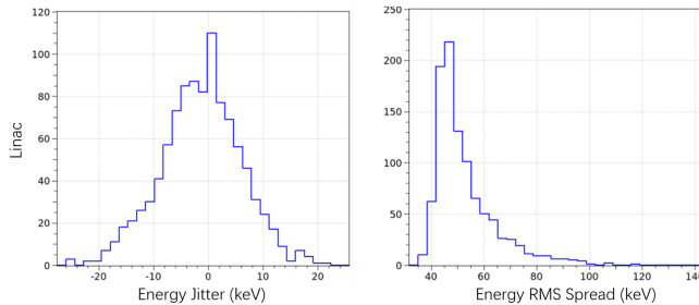
Figure 6: The energy jitter and energy spread after the single debuncher correction
