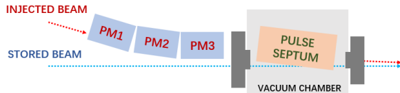
Figure 1: Schematic of the injection setup of a storage ring with septum magnets.
