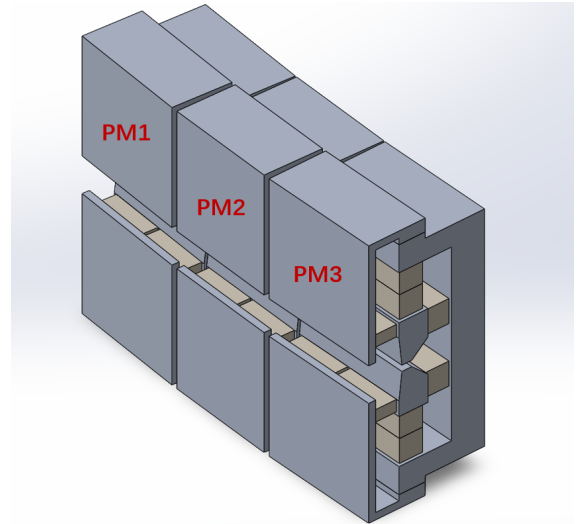
Figure 2: Magnet structure. The brown regions represent Sm_2Co_{17} , whereas the gray regions correspond to DT4 soft iron.
