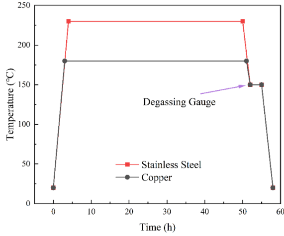
Figure 2: Bakeout procedure for testing setup.
