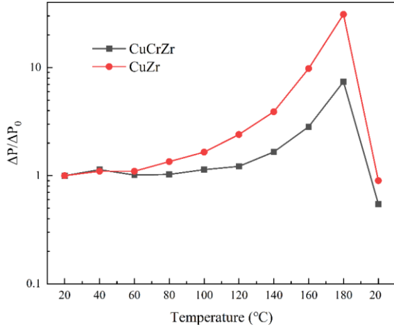
Figure 6: Temperature dependence of the relative pressure change ( \Delta P/\Delta P_0 ) during testing.
