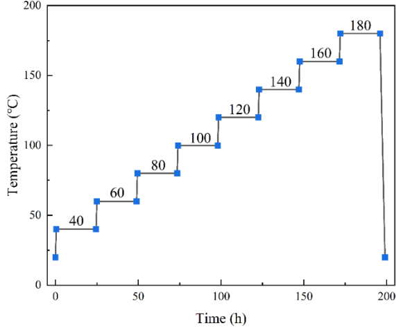
Figure 3: Heating-keeping procedure for copper pipes.
