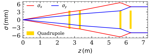
Figure 2: Evolution of the beam through the four-quadrupole configuration.
