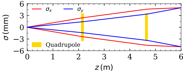
Figure 1: Evolution of the beam through the two-quadrupole configuration.
