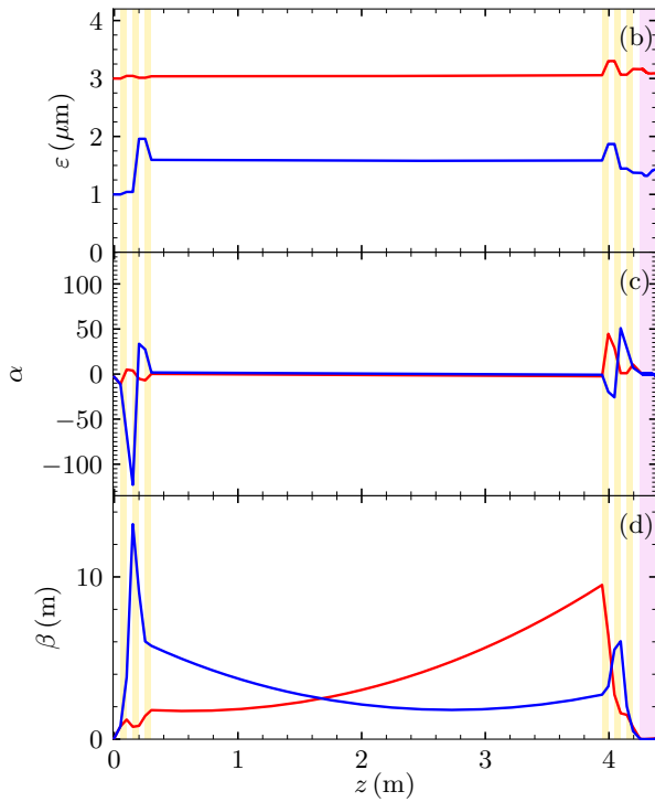
Figure 3: Evolution of the beam through the six-quadrupole configuration and second plasma.
