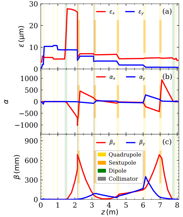
Figure 4: Evolution of the beam through the dogleg configuration.
