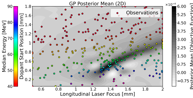
Figure 5: 2D GP Surrogate Model of Dopant Position vs. Longitudinal Laser Focus.
