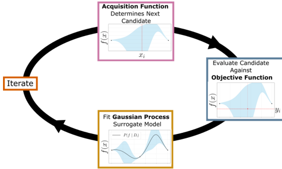
Figure 2: Diagram of a typical Bayesian Optimization loop
