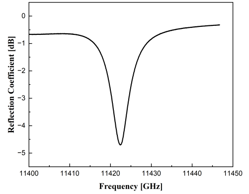
Figure 10: The S parameters for the well-tuned copper prototype.
