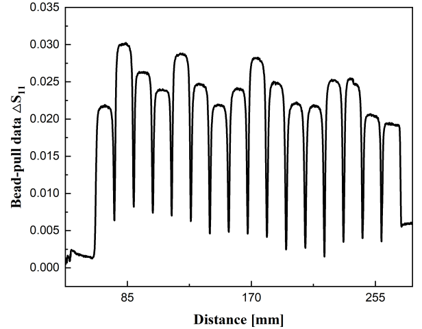
Figure 6: The bead-pull result for the aluminum prototype.
