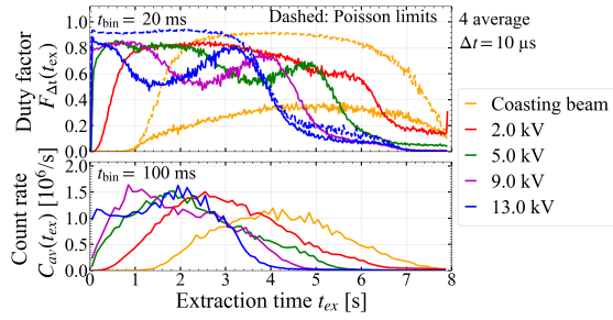
Figure 1: Measured duty factor (top) and count rate (bottom) for \Delta t=10 \mu\text{s} during extraction for different gap voltages, with evaluation interval of t_{\text{bin}} = 20 \text{ ms} and 100 \text{ ms} , respectively.
