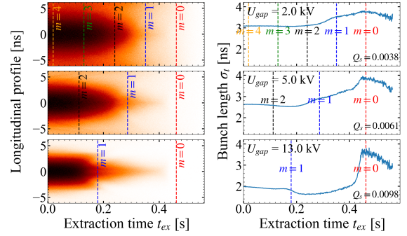
Figure 5: The simulated longitudinal bunch profile evolution of the stored beam. The SBR lines are indicated.
