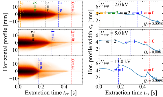
Figure 4: The simulated horizontal profile evolution of the stored beam. The SBRs are marked by lines according to 3Q_x + mQ_s = 13 using the low-amplitude Q_s .
