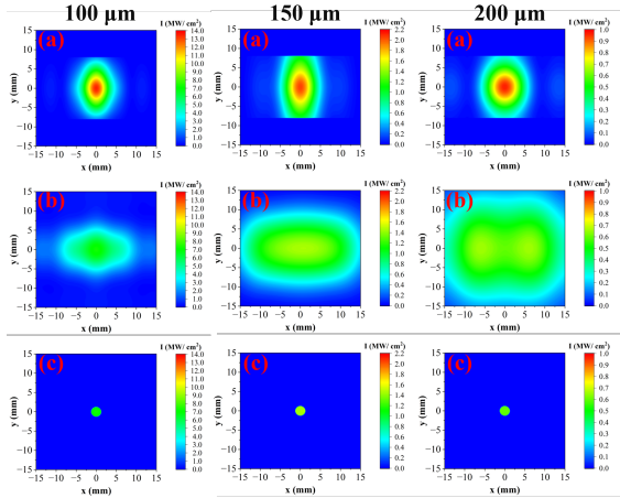
Figure 4: Transverse optical field intensity distributions in HiFEL's partial waveguide cavity.
