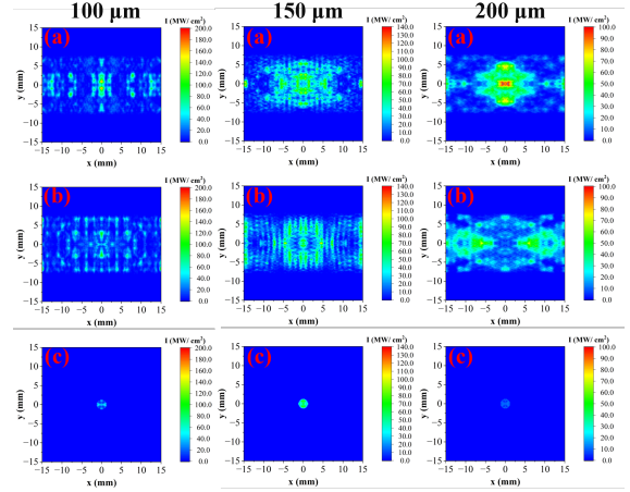
Figure 5: Transverse optical field intensity distributions in HiFEL's full waveguide cavity. It is worth noting that the color scales of Fig. 4 and Fig. 5 are different, with the full waveguide case using a far larger intensity range. We have clarified that the full waveguide design delivers stronger transverse confinement and higher output power, and the seemingly 'better beam' of the partial waveguide is only caused by inconsistent color scale settings, to eliminate misunderstanding.
