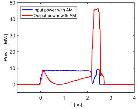
Figure 7: Input and output power waveforms with AM.
