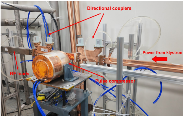
Figure 5: High-power test picture.
