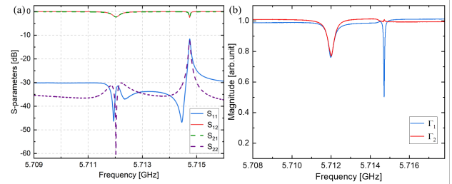
Figure 4: (a) S -parameters and (b) polarized modes after tuning.
