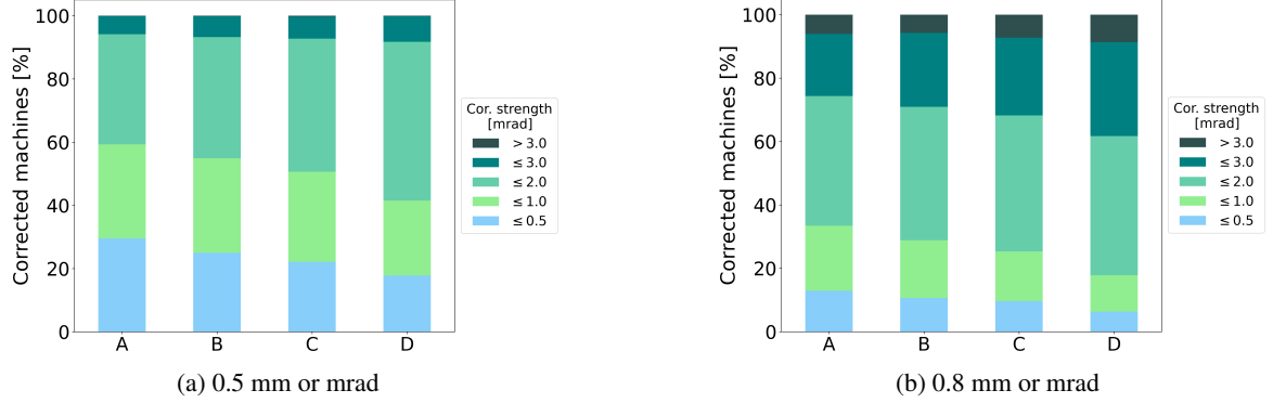
Figure 1: Comparison of maximum corrector strengths required for vertical orbit correction using correction schemes A–D, with misalignment / tilt tolerances of 0.5 and 0.8 mm or mrad. Each color represents the fraction of machines requiring corrector strengths within the ranges specified in the legend.
