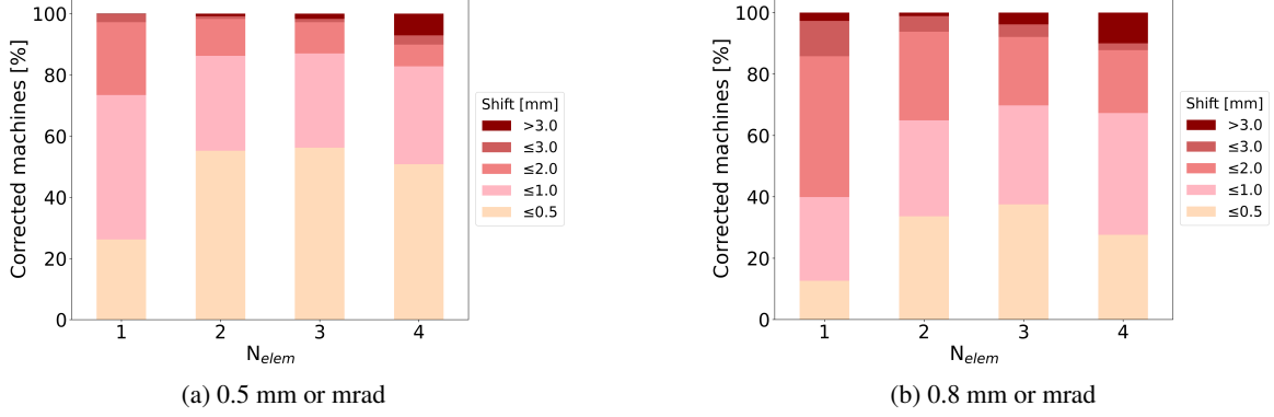
Figure 2: Comparison of maximum realignment shifts required for vertical orbit correction via beam-based quadrupole alignment with 1–4 elements, for misalignment / tilt tolerances of 0.5 and 0.8 mm or mrad. Each color represents the fraction of machines requiring shifts within the ranges specified in the legend.
