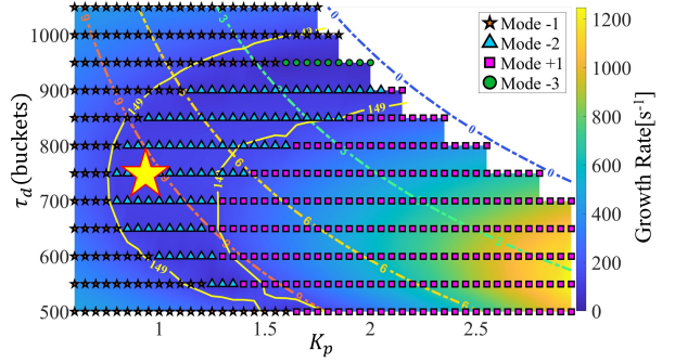
Figure 2: Stability map for STCF at 3.5 GeV in the (K_P, \tau_d) plane. The color scale represents the growth rate of the fastest-growing mode, with markers indicating the mode index (stars: mode -1 ; triangles: mode -2 ; squares: mode +1 ). The solid contour labeled "149" marks the radiation damping threshold 1/\tau_{\text{rad}} , while dashed contours denote the gain margin. The white upper-right region is excluded by the Nyquist criterion. The parameter set (K_P, \tau_d) = (1, 750) buckets is selected as an illustrative initial commissioning setting.
