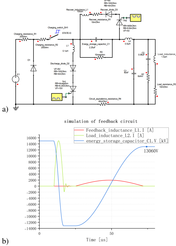
Figure 3: Simulation of the feedback circuit. (a) Simulation diagram. (b) Simulated results.
