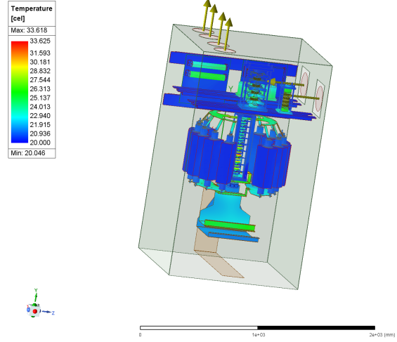
Figure 4: Heat dissipation simulation of cabinet interior.
