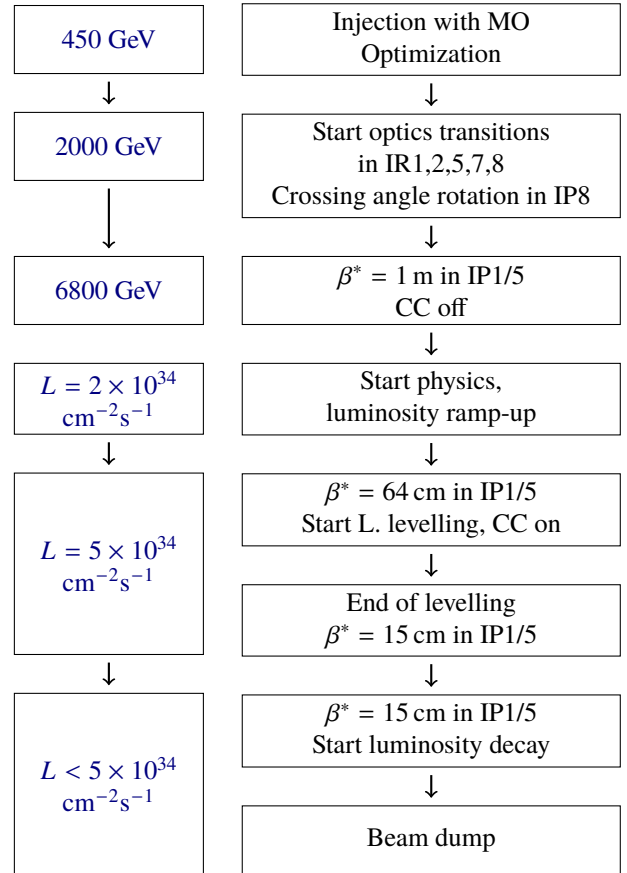
Figure 4: Main steps of the nominal HL-LHC cycle.
