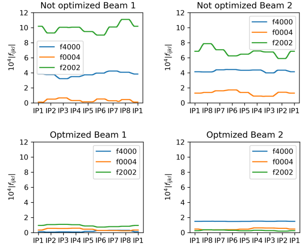
Figure 1: Optimisation of the octupolar resonance driving term at injection for Beam 1 and Beam 2. The plots show the amplitude of the first-order octupolar resonance driving terms (for the definition refer to [17]) in the lattice for the previous HL-LHC baseline injection optics and the newly proposed injection optics. The reduction of the perturbation is significant for both beams.
