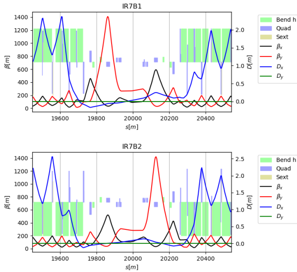
Figure 3: Optimised collimation insertion optics for Beam 1 and Beam 2. Compared with the reference optics, the large \beta -functions are not compatible with the aperture at injection energy; therefore, an optics transition is needed.
