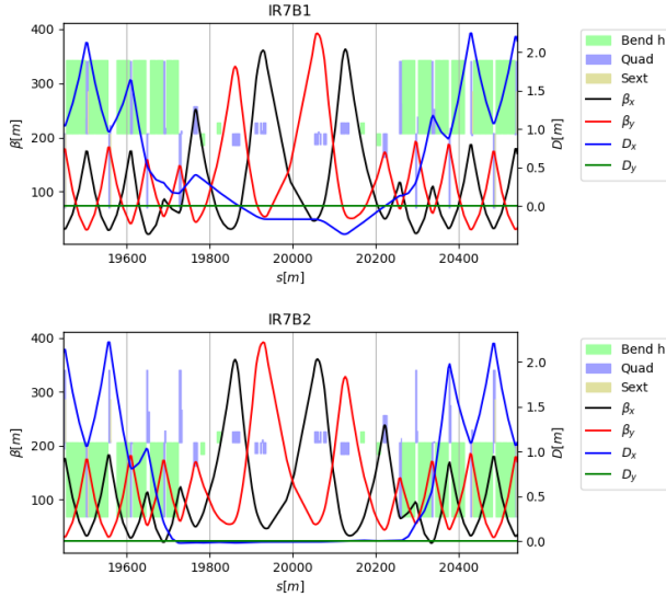
Figure 2: Reference collimation insertion optics for Beam 1 and Beam 2. The plots show the Twiss parameters and dispersion in the area together with the position and strengths of the the main magnets, shown without units.
