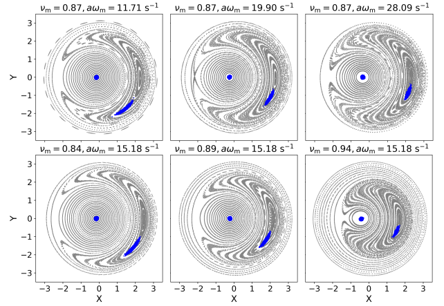
Figure 1: Phase-space portraits of the Hamiltonian (4) using X = \sqrt{2I} \cos \theta , Y = \sqrt{2I} \sin \theta vs. \nu_m and a\omega_m . Equilibrium distributions (blue) from Eqs. (10) are also shown. We remark the the damping effect breaks the Y -symmetry of the system as it clearly visible from the fixed point displacement.
