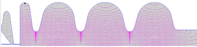
Figure 4: Field map of 3.5 cells superconducting RF Gun calculated by Superfish.
