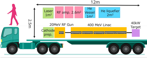
Figure 7: A layout of the portable muon source based on superconducting linac operated at 4 K.
