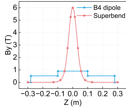
Figure 2: Longitudinal field profiles of the conventional B4 dipole and an illustrative superbend.
