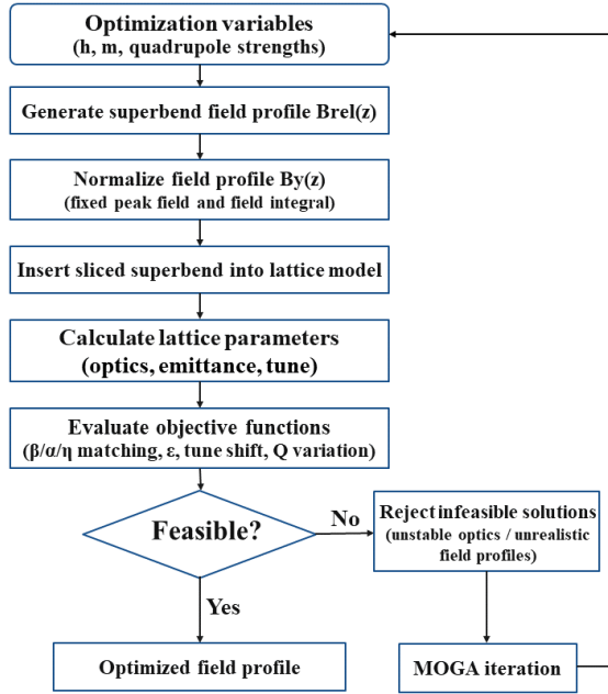
Figure 3: Flowchart of the multi-objective optimization and lattice rematching procedure.
