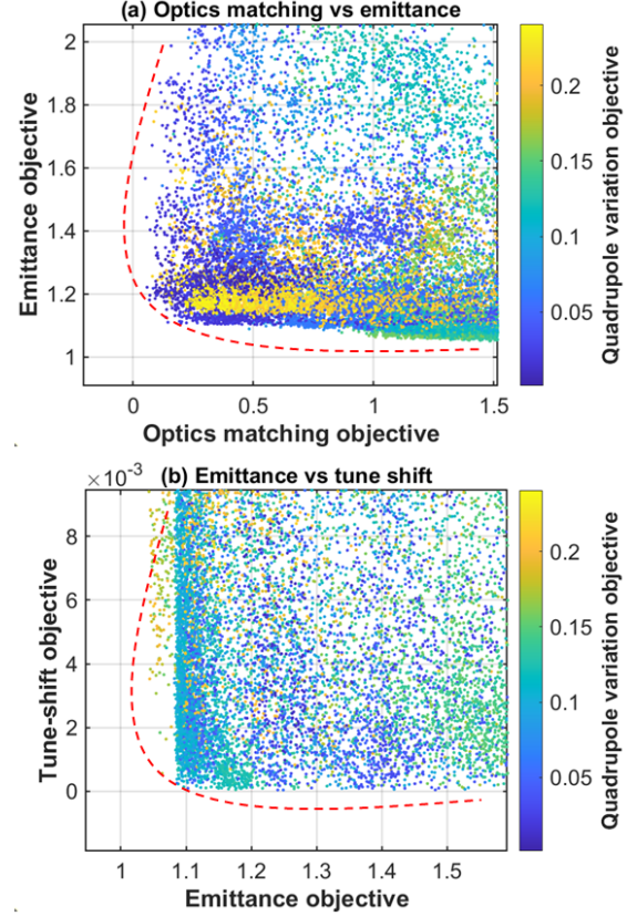
Figure 4: Two-dimensional Pareto-front projections of the multi-objective optimization results: (a) optics-matching objective versus emittance objective, with quadrupole variation indicated by color; (b) emittance objective versus tune-shift objective, with quadrupole variation indicated by color.
