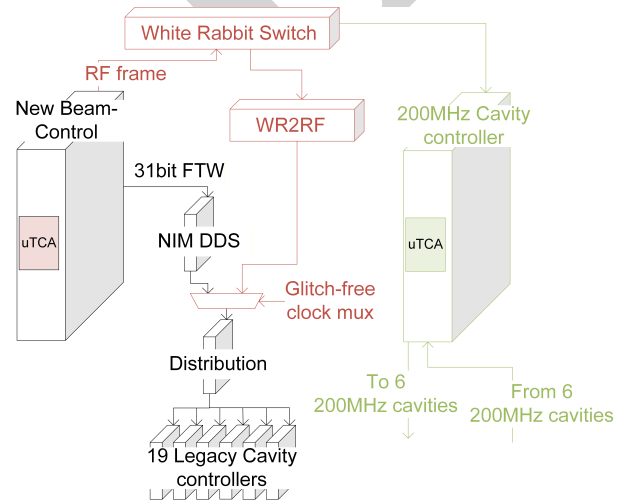
Figure 4: Layout of proposed WR distribution.
