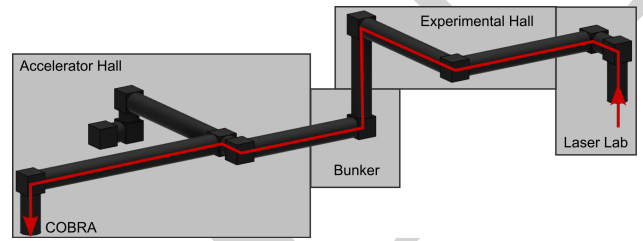
Figure 4: The laser beam transport line from the laser laboratory to the accelerator hall. The laser (red) is deflected by highly reflective mirrors. The empty path of the beam-line directs to the laser driven electron photogun of the S-DALINAC. Adapted from Ref. [12]
