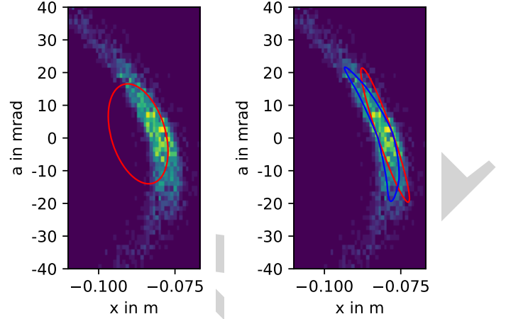
(a) Linear phase space (red) from (b) Linear (red) and quadratic mean and covariance phase space from generalized Irwin model.
