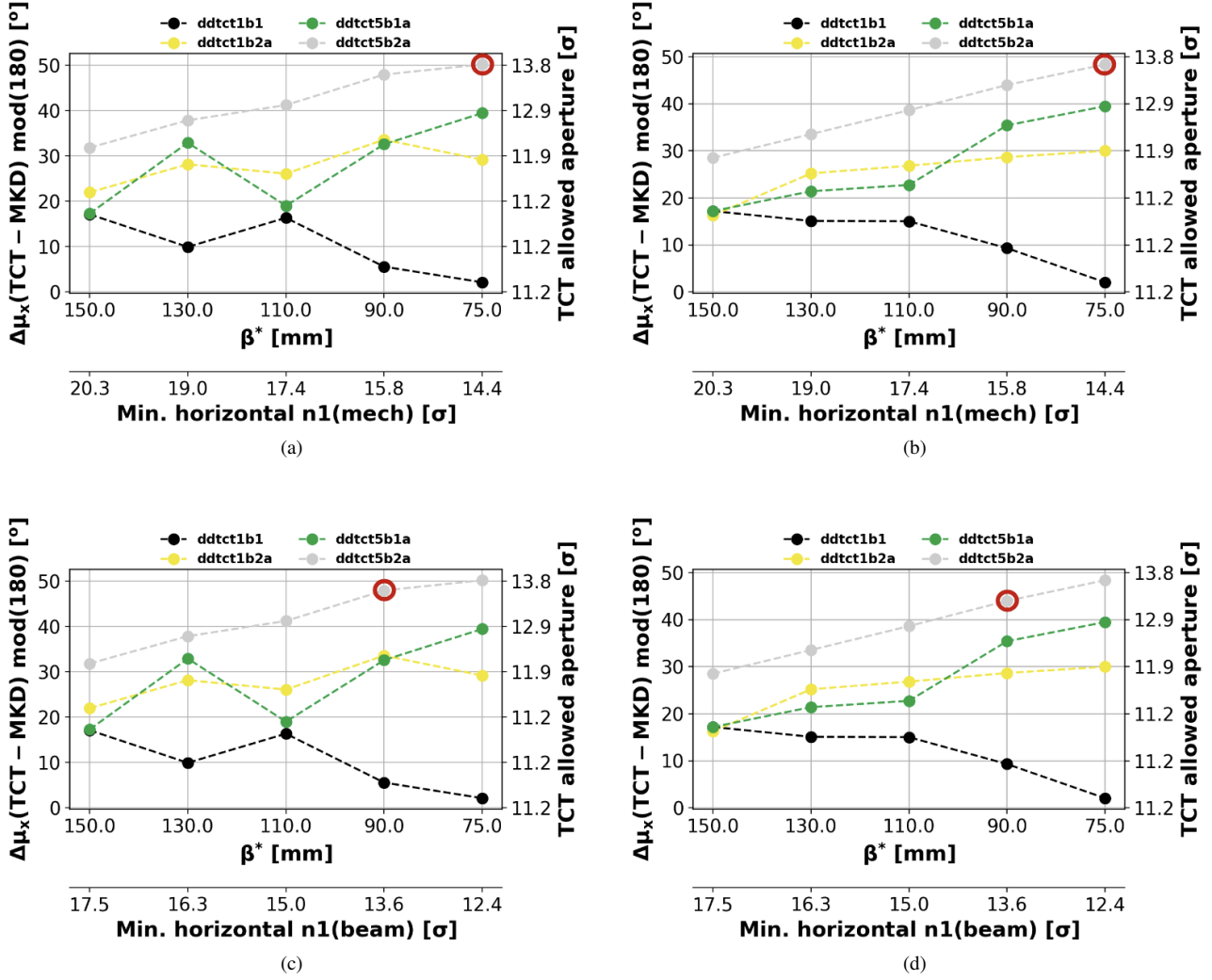
Figure 2: TCT-MKD phase advance and allowed aperture for different \beta^* values in the parallel plane for 470 m \beta_x at TCDQ (a, c) and 430 m \beta_x at TCDQ (b, d). The bottom x-axis represents the protected aperture under different imperfection scenarios ( mech for top row, beam for bottom row). The TCT allowed aperture must be smaller than the protected one; red circles indicate the most performance-oriented optics achieved.
