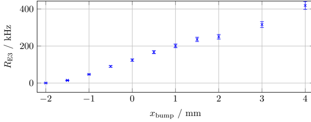
Figure 4: Rate R_{E3} of extracted electrons at E3 beamline in dependence of the magnitude of the closed orbit bump x_{\text{bump}} .
