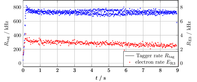
Figure 6: Event rate of tagged electrons at CB-ELSA/TAPS experiment ( R_{\text{tag}} ) and simultaneous electron rate at the detector test beamline ( R_{E3} ).
