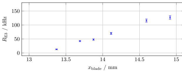
Figure 5: Rate R_{E3} of extracted electrons at E3 beamline in dependence of the septum blade position x_{\text{blade}} .
