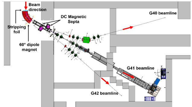
Figure 1: Schematic view of the three beamlines dedicated to the industrial applications at GANIL. The middle beamline is already in use, the others are in study.
